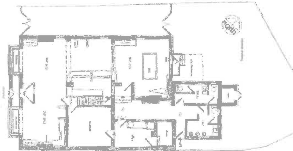
Proposed ground floor layout 4.1.1.1 79 sqm
